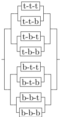
Figure 7: Parallel blocks in parallel, in parallel
